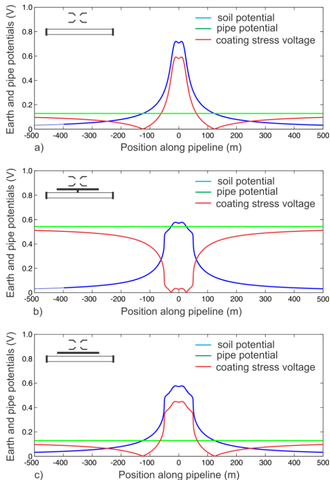
Fig.4. Soil potential, pipe potential and coating stress voltage in three scenarios:a) without using mitigation, b) with 100m FeZn ribbon in the same trench with pile and connected to pipe, c) with 100 m FeZn ribbon detached from pipe (normalized values per dissipated current of 1 A through the tower grounding)
