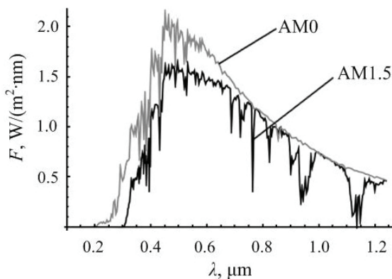
Fig.2. Spectral solar irradiance [18, 19]
