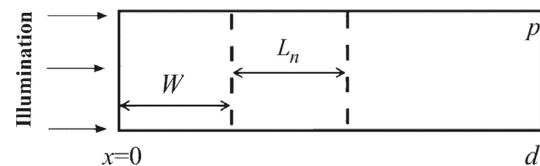
Fig.1. One-dimensional model of SC CIGSS-layer: W – the SCR value, L_n – the diffusion length, d – the thickness of CIGSS-layer
