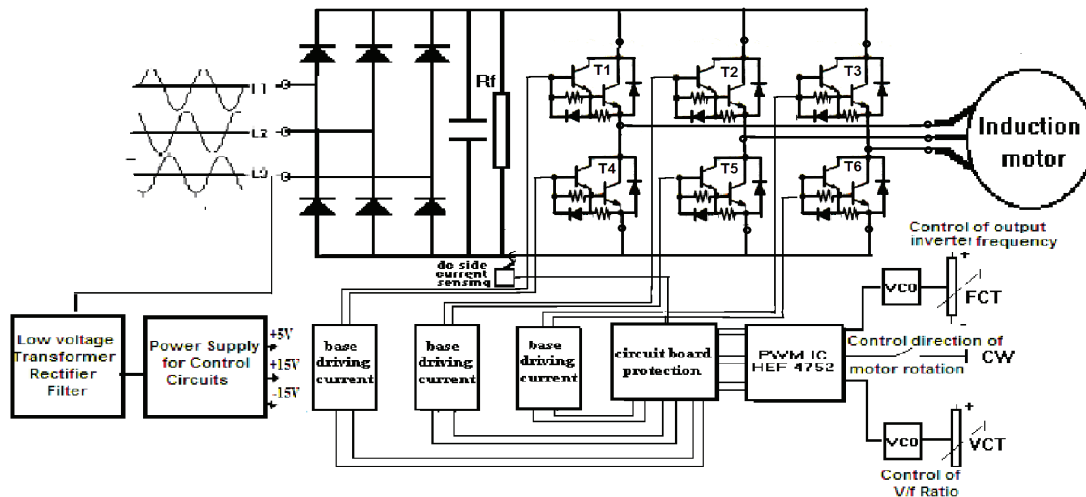
Fig.1 Block Diagram of the control system
