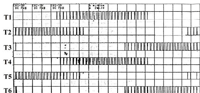
Fig.6 Experimental waveforms of the three complementary pairs of inverter drive signals
