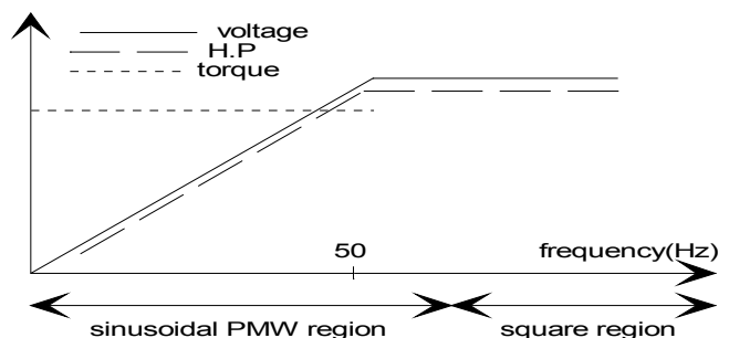
Fig.4 Motor torque capability
