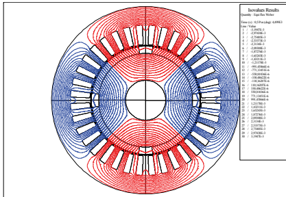
Fig.1. Distribution of magnetic flux density in PM machine obtained by FLUX simulation software
