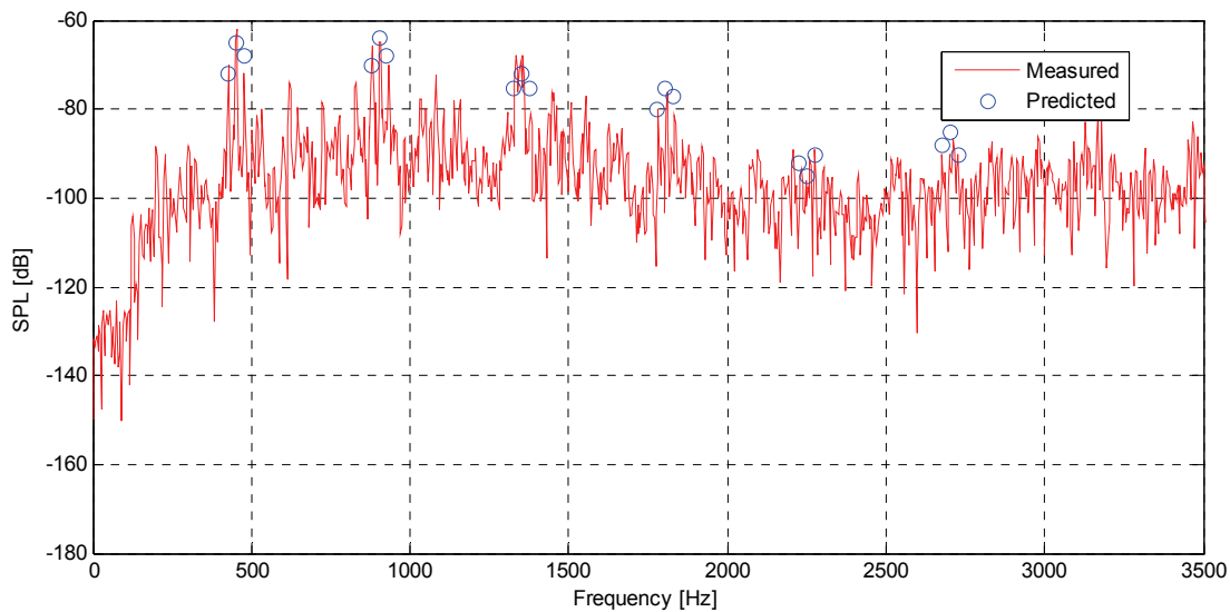
Fig.12 Noise spectrum of the machine under test with disk (with eccentricity)
