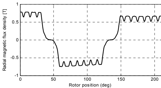
Fig.4. Air-gap magnetic flux density with 0% eccentricity
