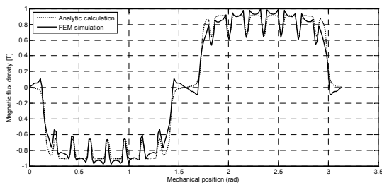
Fig.2. Magnetic flux density in the air-gap of the motor
