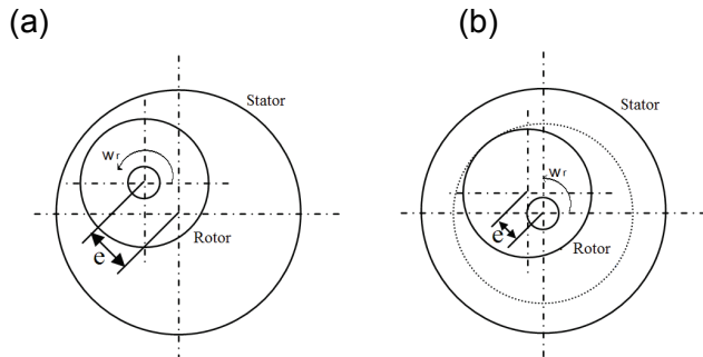
Fig.3. Rotor eccentricity (a) static, (b) dynamic
