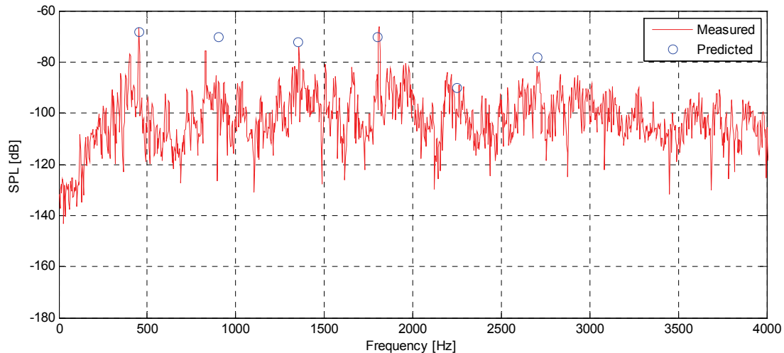
Fig.11 Noise spectrum of the machine under test without disk (without eccentricity)
