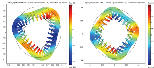
Fig.6. Order 3 (left) and order 4 (right) of PMSM
