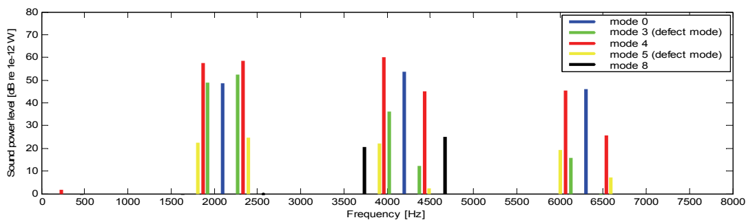
Fig.8. Sound power level spectrum at 3500 rpm and with 25 % eccentricity
